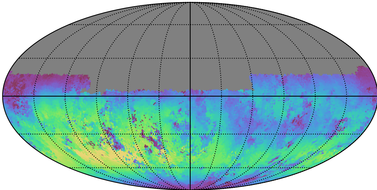
weather_cloudso4v3.4_10yrs Yr 1 u band: Median skyBrightness
