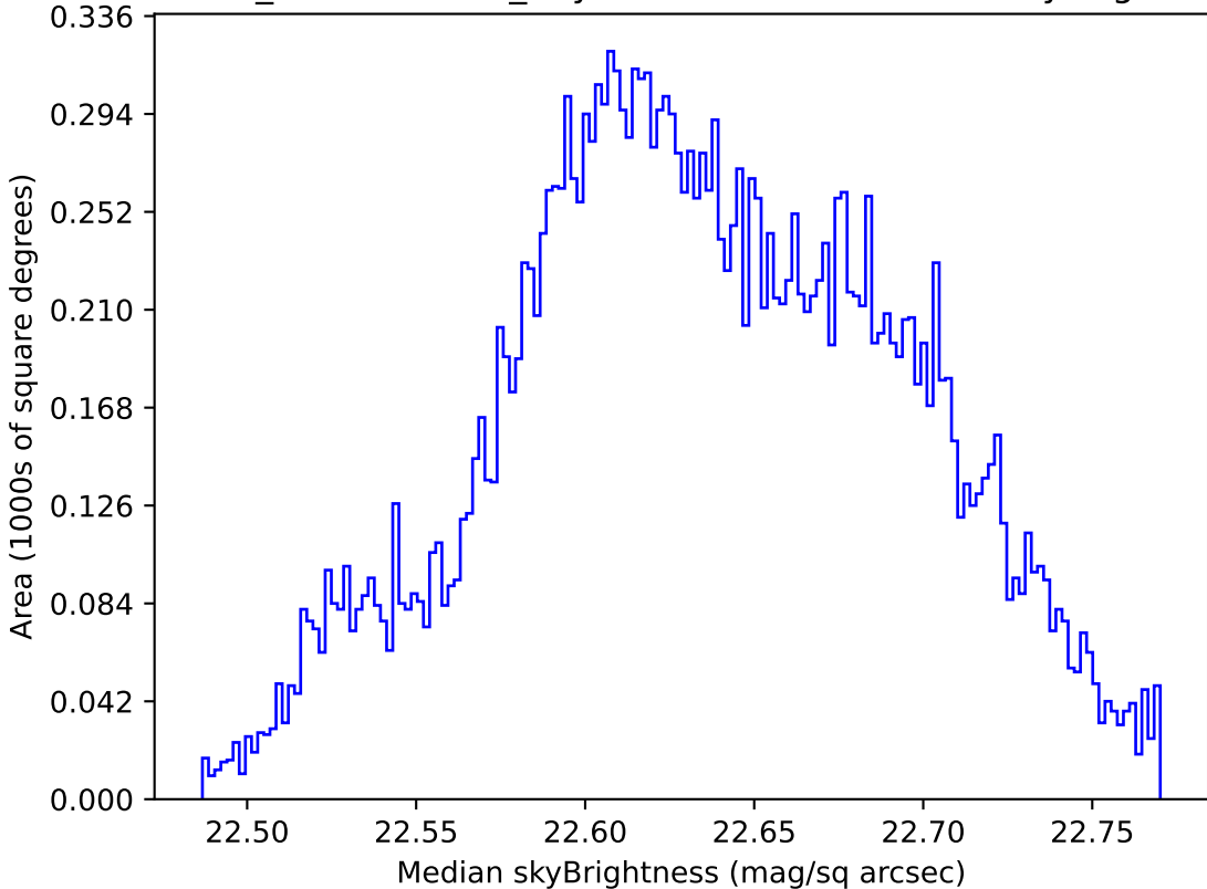
weather_cloudso4v3.4_10yrs Yr 1 u band: Median skyBrightness
