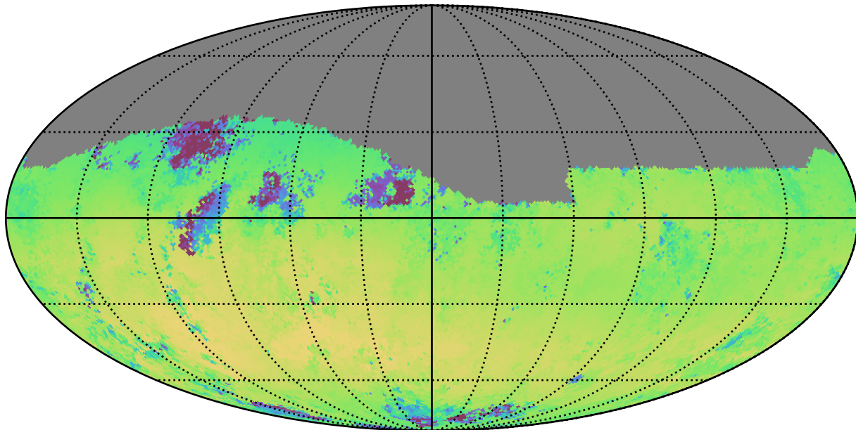
weather_cloudso4v3.4_10yrs Yr 1 r band: Median skyBrightness
