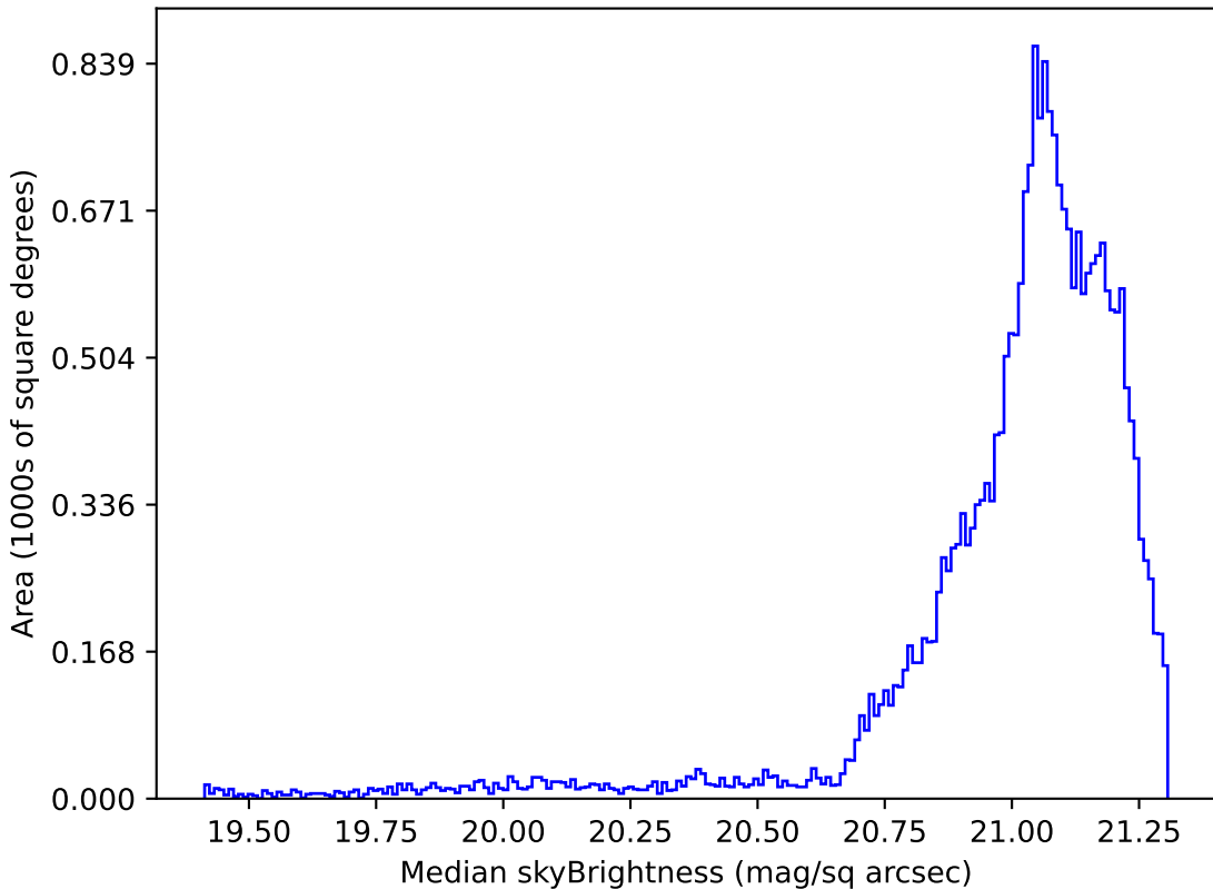
weather_cloudso4v3.4_10yrs Yr 1 r band: Median skyBrightness
