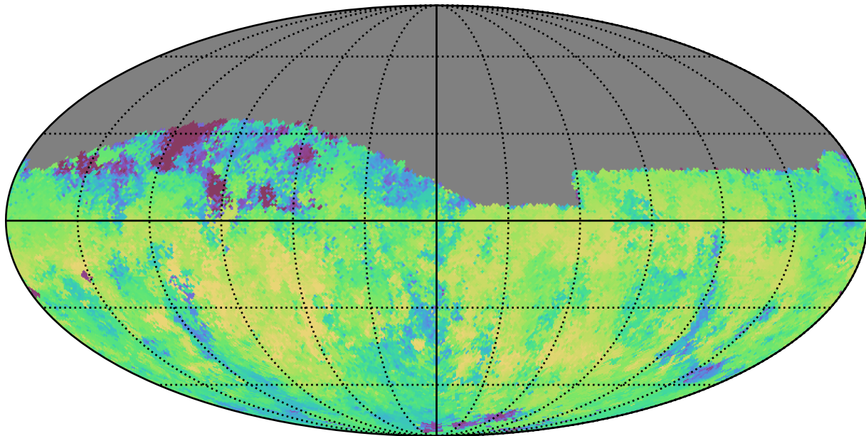
weather_cloudso4v3.4_10yrs Yr 1 i band: Median skyBrightness
