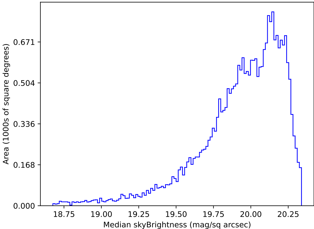
weather_cloudso4v3.4_10yrs Yr 1 i band: Median skyBrightness
