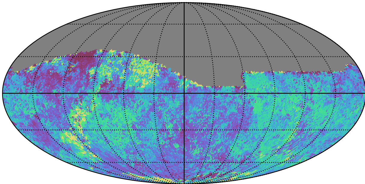
weather_cloudso4v3.4_10yrs Yr 1 all bands: Median skyBrightness
