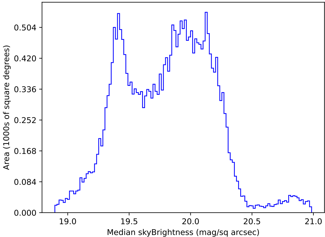
weather_cloudso4v3.4_10yrs Yr 1 all bands: Median skyBrightness
