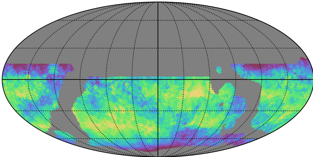
weather_cloudso4v3.4_10yrs WFD z band: Median skyBrightness
