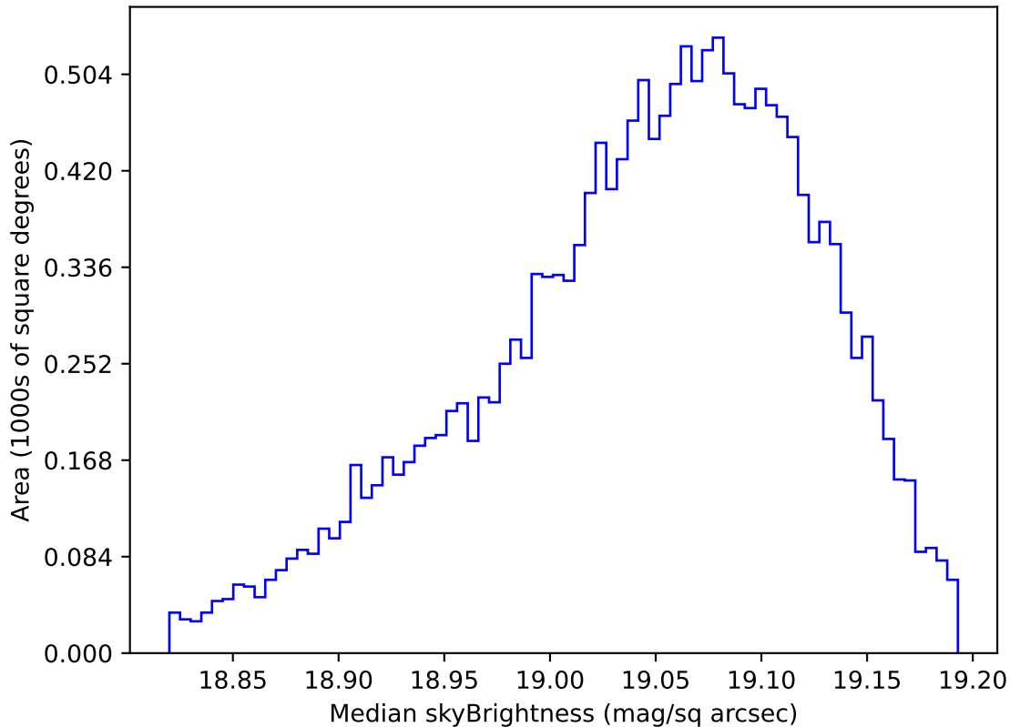
weather_cloudso4v3.4_10yrs WFD z band: Median skyBrightness
