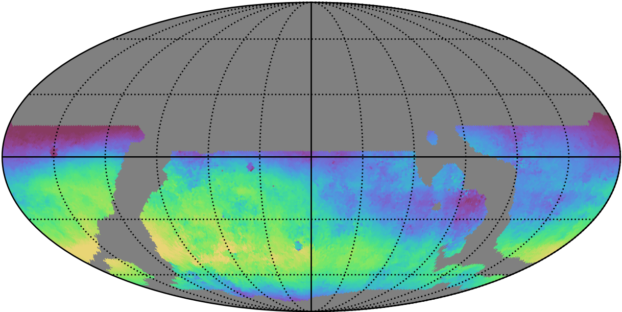
weather_cloudso4v3.4_10yrs WFD u band: Median skyBrightness
