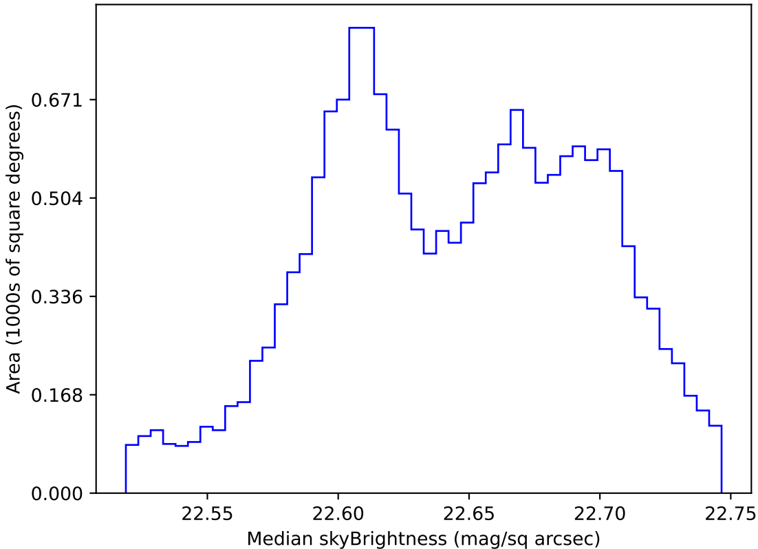
weather_cloudso4v3.4_10yrs WFD u band: Median skyBrightness
