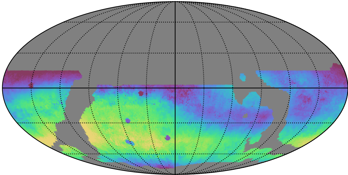
weather_cloudso4v3.4_10yrs WFD r band: Median skyBrightness
