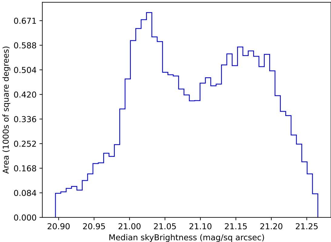
weather_cloudso4v3.4_10yrs WFD r band: Median skyBrightness
