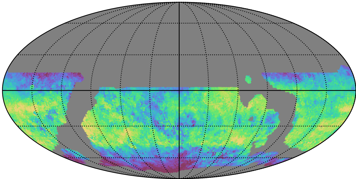
weather_cloudso4v3.4_10yrs WFD i band: Median skyBrightness
