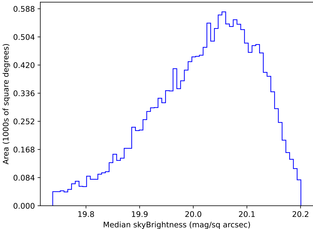
weather_cloudso4v3.4_10yrs WFD i band: Median skyBrightness
