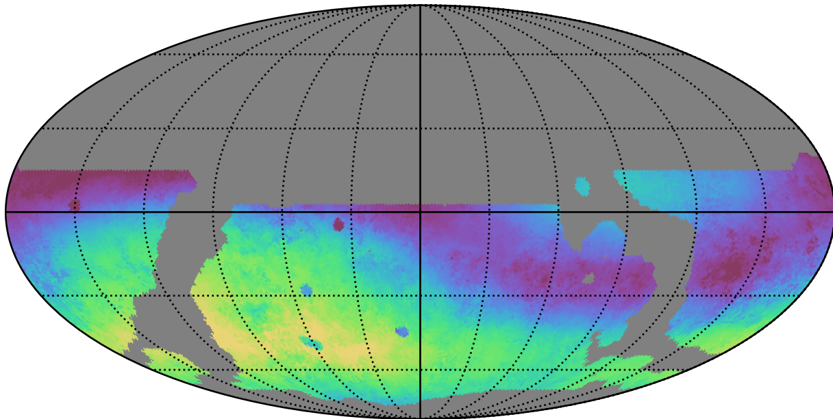
weather_cloudso4v3.4_10yrs WFD g band: Median skyBrightness
