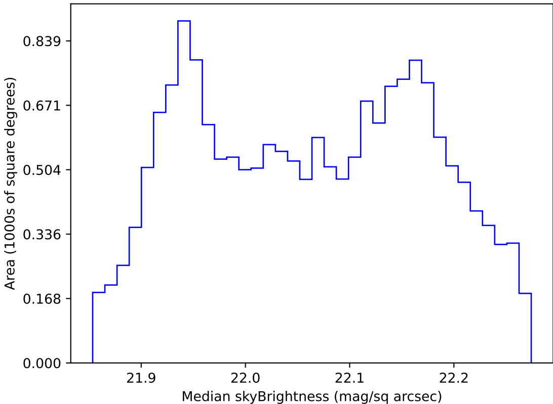
weather_cloudso4v3.4_10yrs WFD g band: Median skyBrightness
