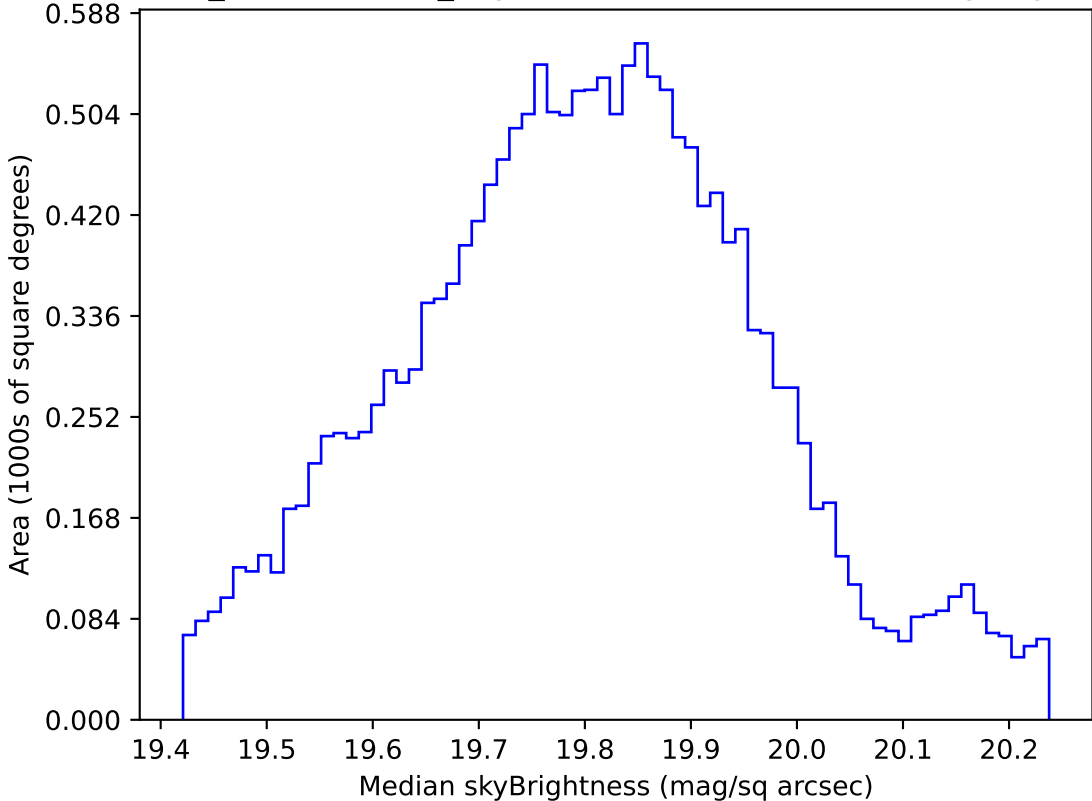
weather_cloudso4v3.4_10yrs WFD all bands: Median skyBrightness
