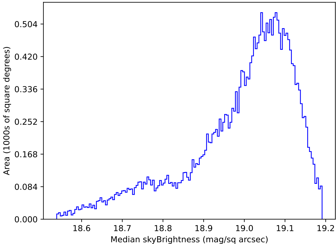
weather_cloudso4v3.4_10yrs All sky z band: Median skyBrightness
