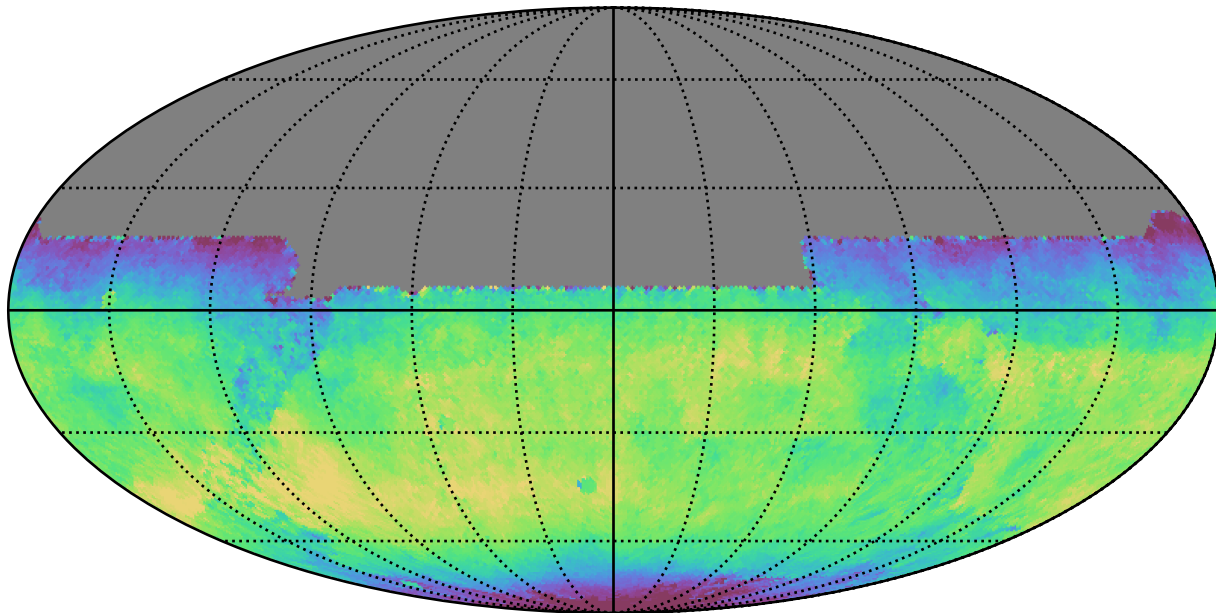
weather_cloudso4v3.4_10yrs All sky y band: Median skyBrightness
