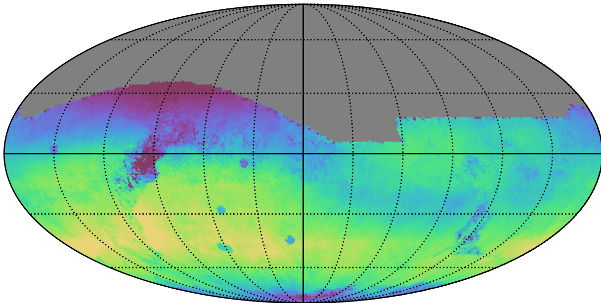
weather_cloudso4v3.4_10yrs All sky r band: Median skyBrightness
