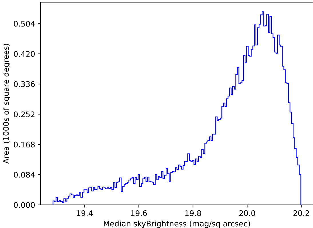
weather_cloudso4v3.4_10yrs All sky i band: Median skyBrightness
