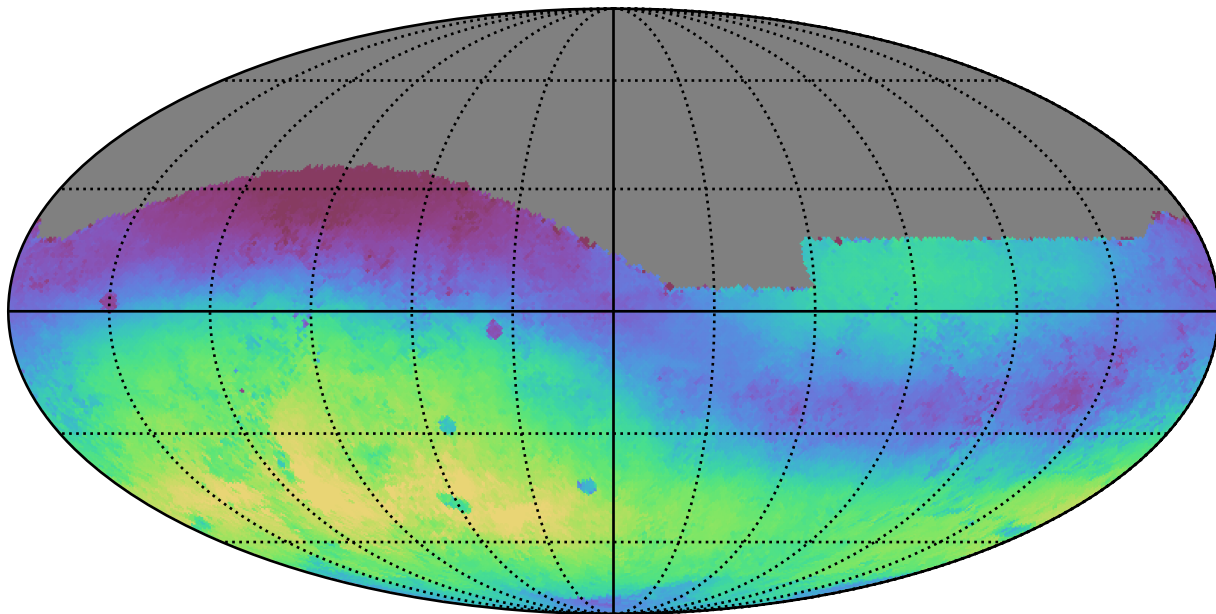
weather_cloudso4v3.4_10yrs All sky g band: Median skyBrightness
