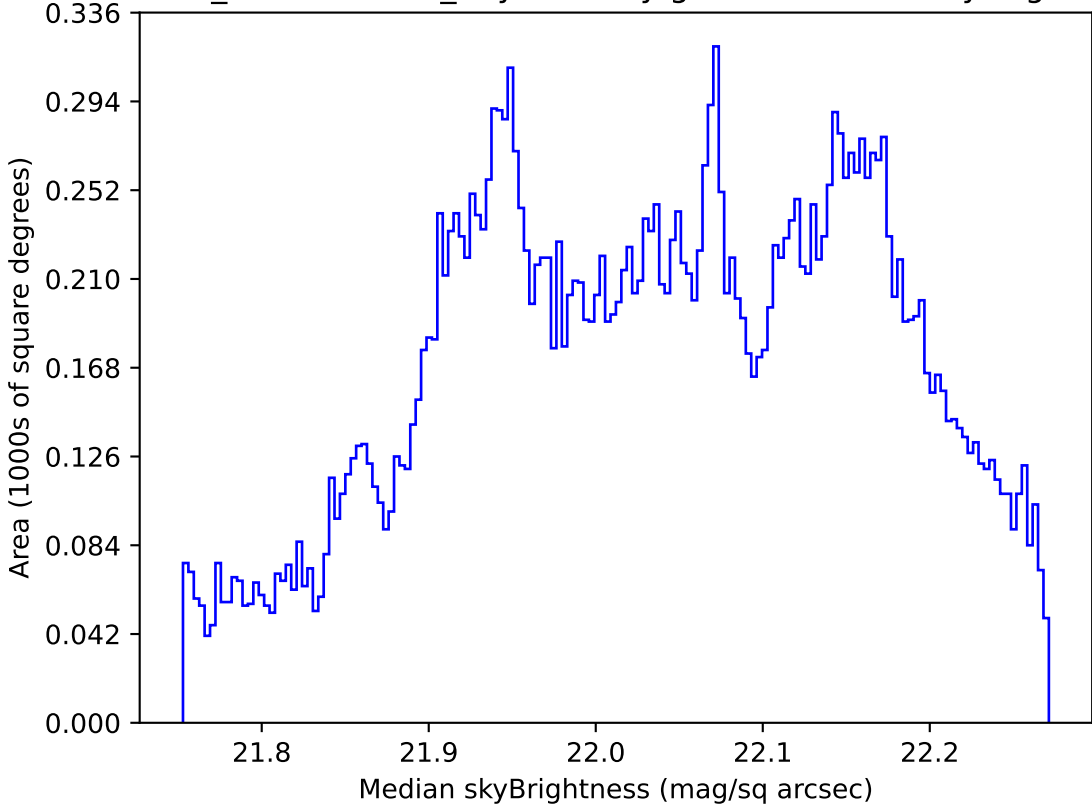
weather_cloudso4v3.4_10yrs All sky g band: Median skyBrightness
