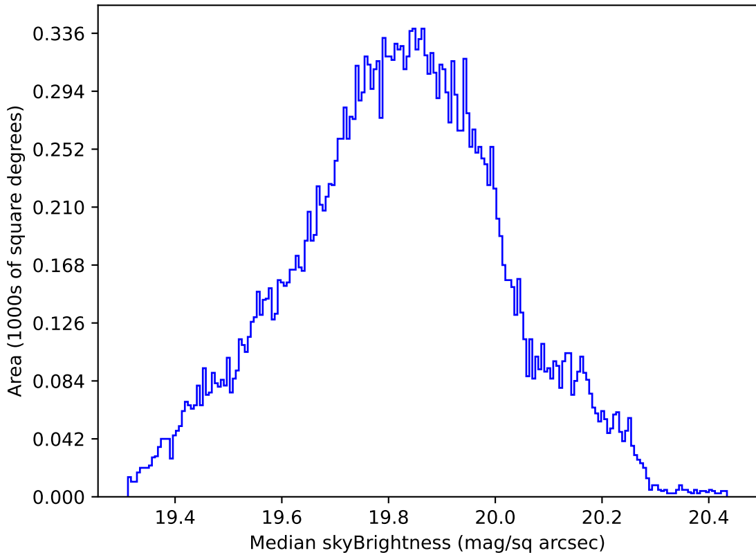
weather_cloudso4v3.4_10yrs All sky all bands: Median skyBrightness
