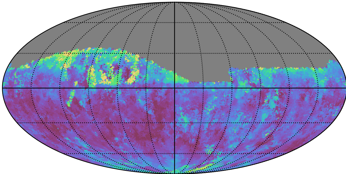
weather_cloudso4v3.4_10yrs Yr 1 z band: Median seeingGeom
