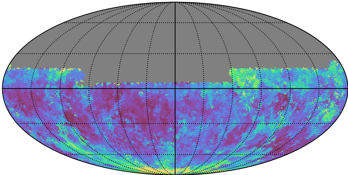
weather_cloudso4v3.4_10yrs Yr 1 y band: Median seeingGeom
