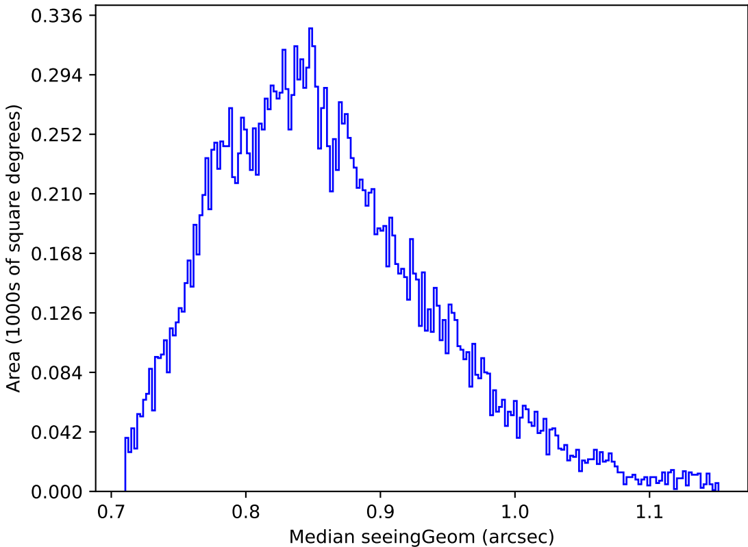
weather_cloudso4v3.4_10yrs Yr 1 y band: Median seeingGeom
