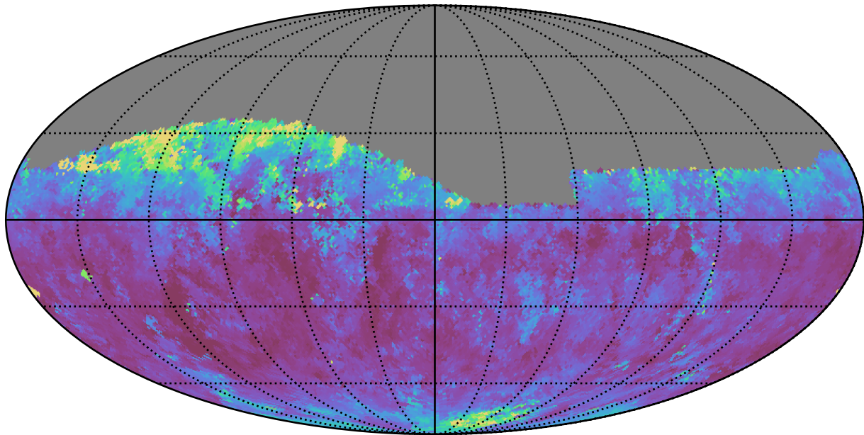
weather_cloudso4v3.4_10yrs Yr 1 i band: Median seeingGeom
