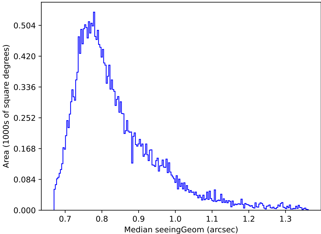
weather_cloudso4v3.4_10yrs Yr 1 i band: Median seeingGeom
