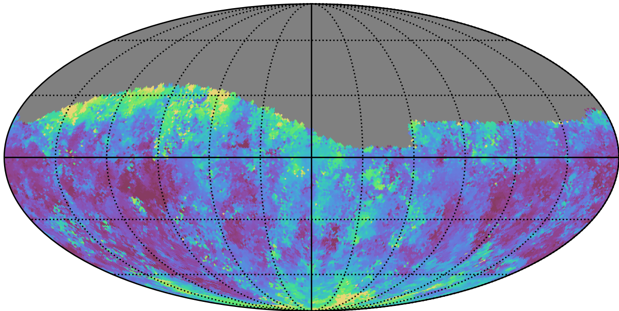
weather_cloudso4v3.4_10yrs Yr 1 g band: Median seeingGeom
