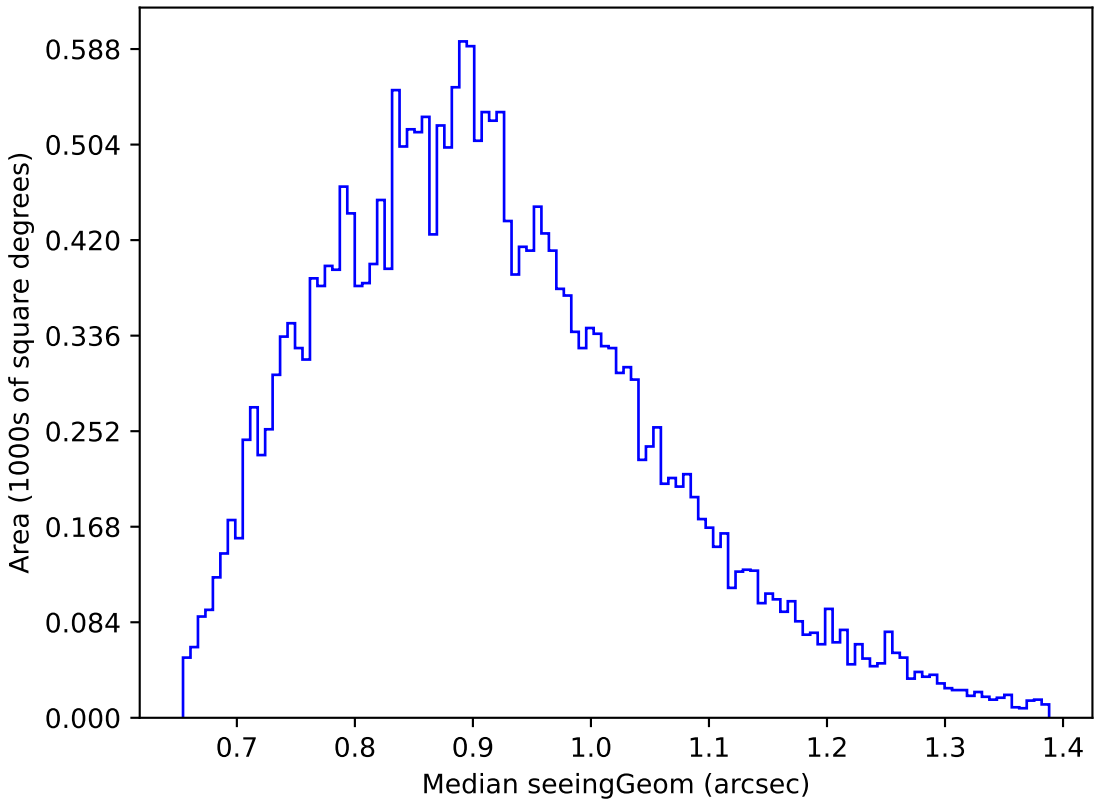
weather_cloudso4v3.4_10yrs Yr 1 g band: Median seeingGeom
