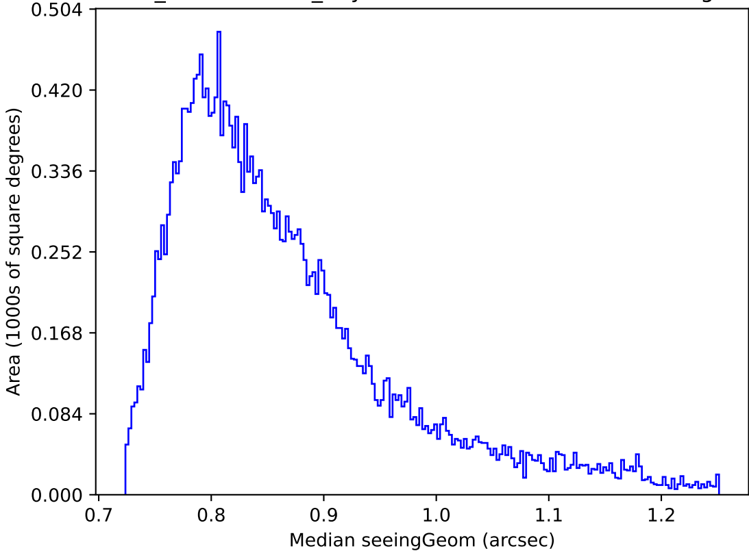
weather_cloudso4v3.4_10yrs Yr 1 all bands: Median seeingGeom
