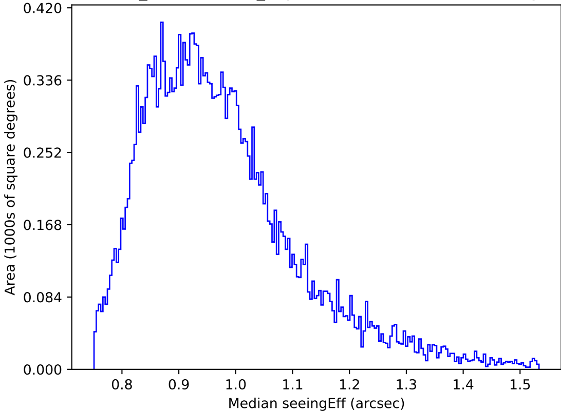
weather_cloudso4v3.4_10yrs Yr 1 z band: Median seeingEff
