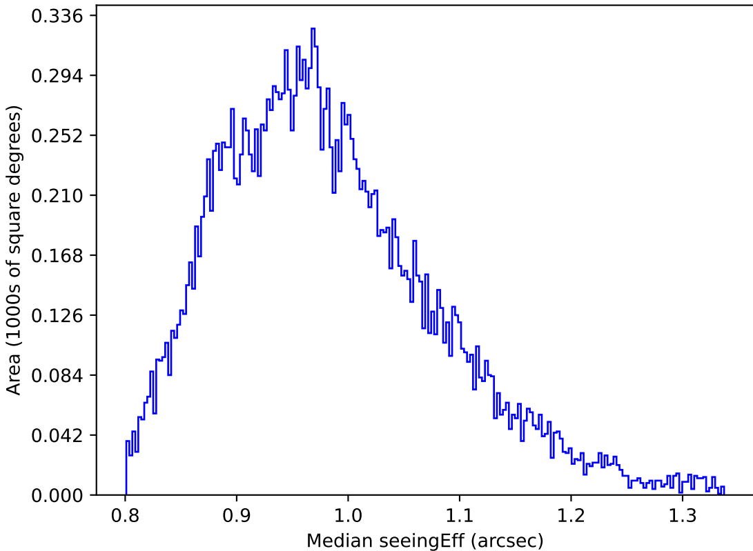
weather_cloudso4v3.4_10yrs Yr 1 y band: Median seeingEff
