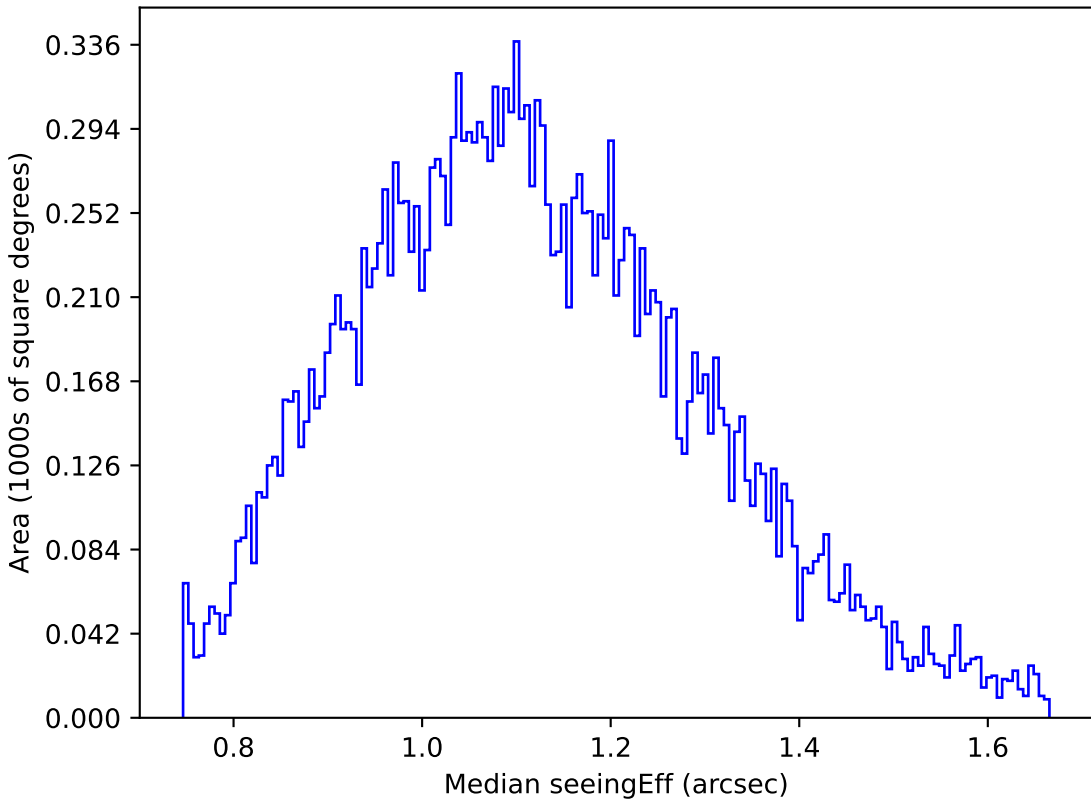
weather_cloudso4v3.4_10yrs Yr 1 u band: Median seeingEff
