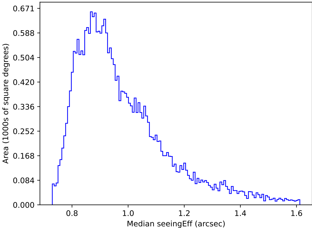
weather_cloudso4v3.4_10yrs Yr 1 r band: Median seeingEff
