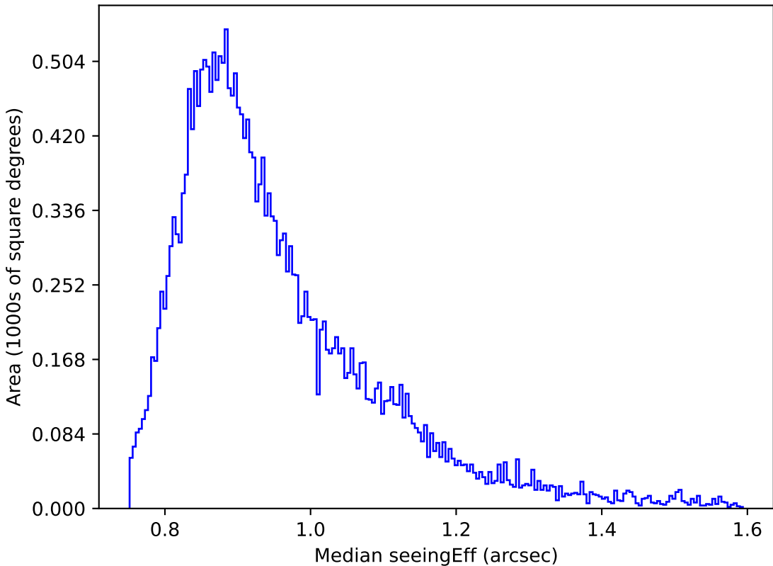
weather_cloudso4v3.4_10yrs Yr 1 i band: Median seeingEff
