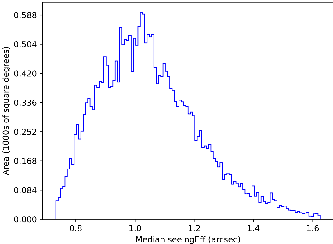
weather_cloudso4v3.4_10yrs Yr 1 g band: Median seeingEff
