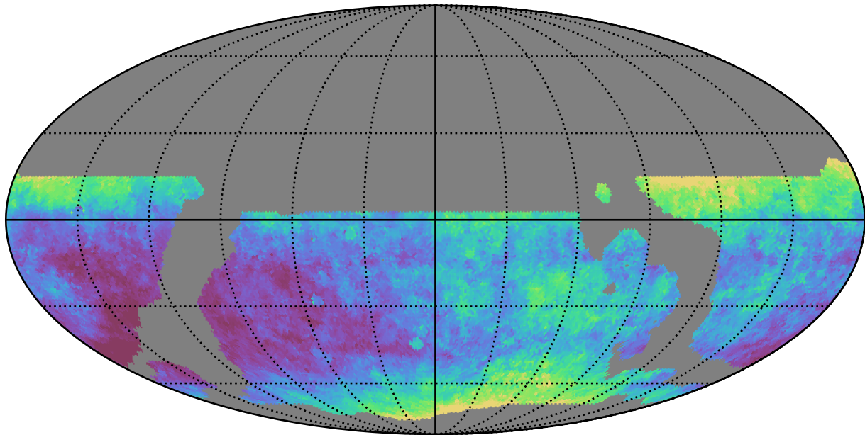
weather_cloudso4v3.4_10yrs WFD z band: Median seeingEff
