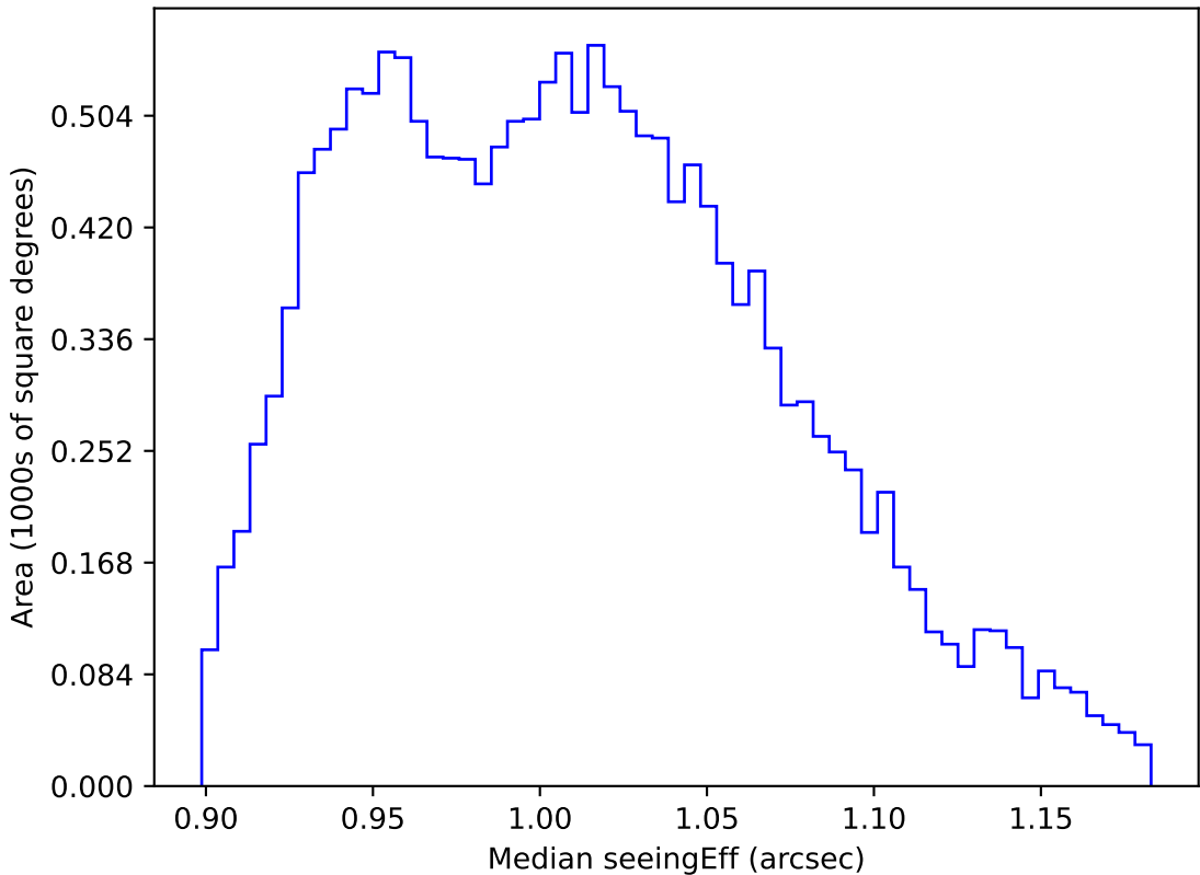
weather_cloudso4v3.4_10yrs WFD y band: Median seeingEff
