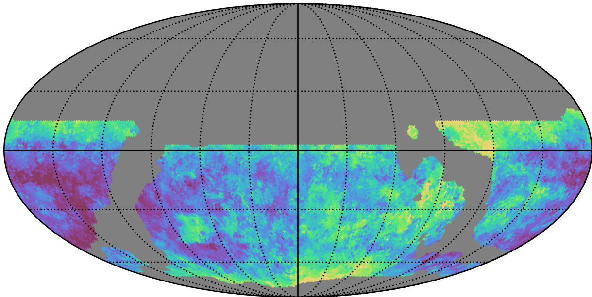
weather_cloudso4v3.4_10yrs WFD u band: Median seeingEff
