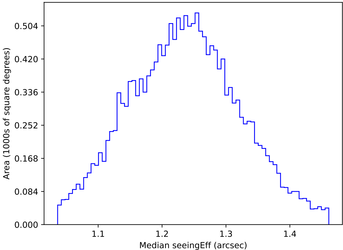
weather_cloudso4v3.4_10yrs WFD u band: Median seeingEff
