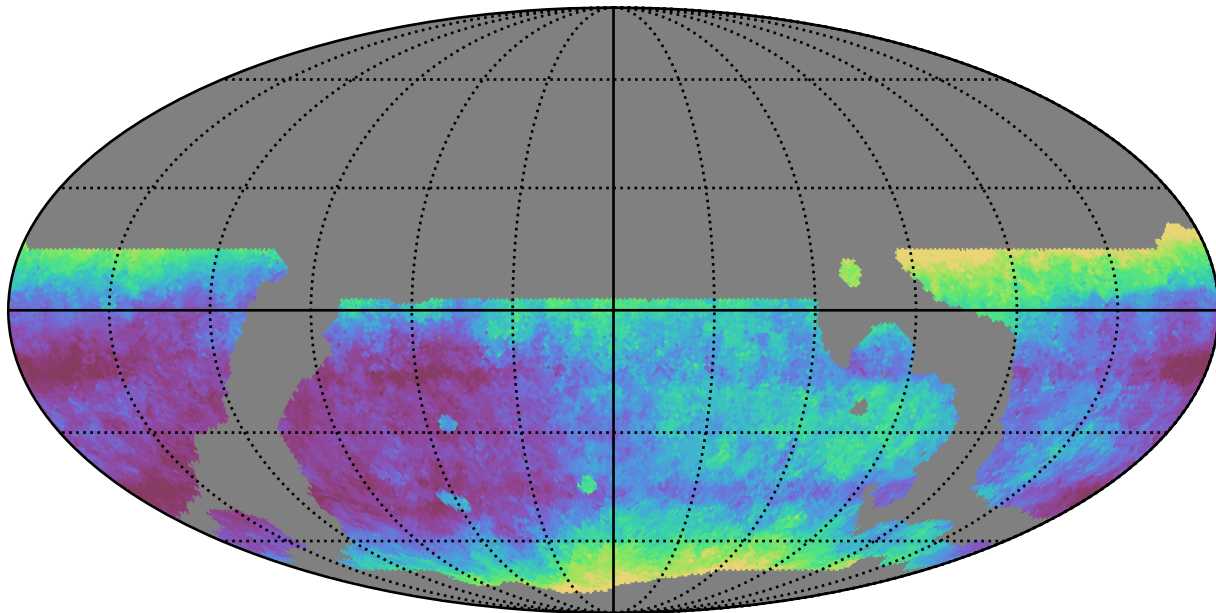
weather_cloudso4v3.4_10yrs WFD r band: Median seeingEff
