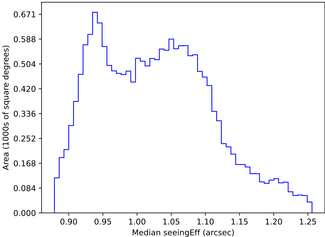
weather_cloudso4v3.4_10yrs WFD r band: Median seeingEff
