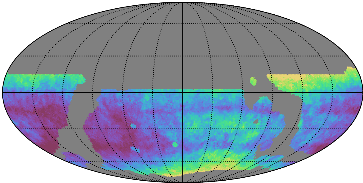
weather_cloudso4v3.4_10yrs WFD i band: Median seeingEff
