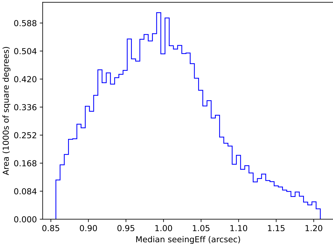
weather_cloudso4v3.4_10yrs WFD i band: Median seeingEff
