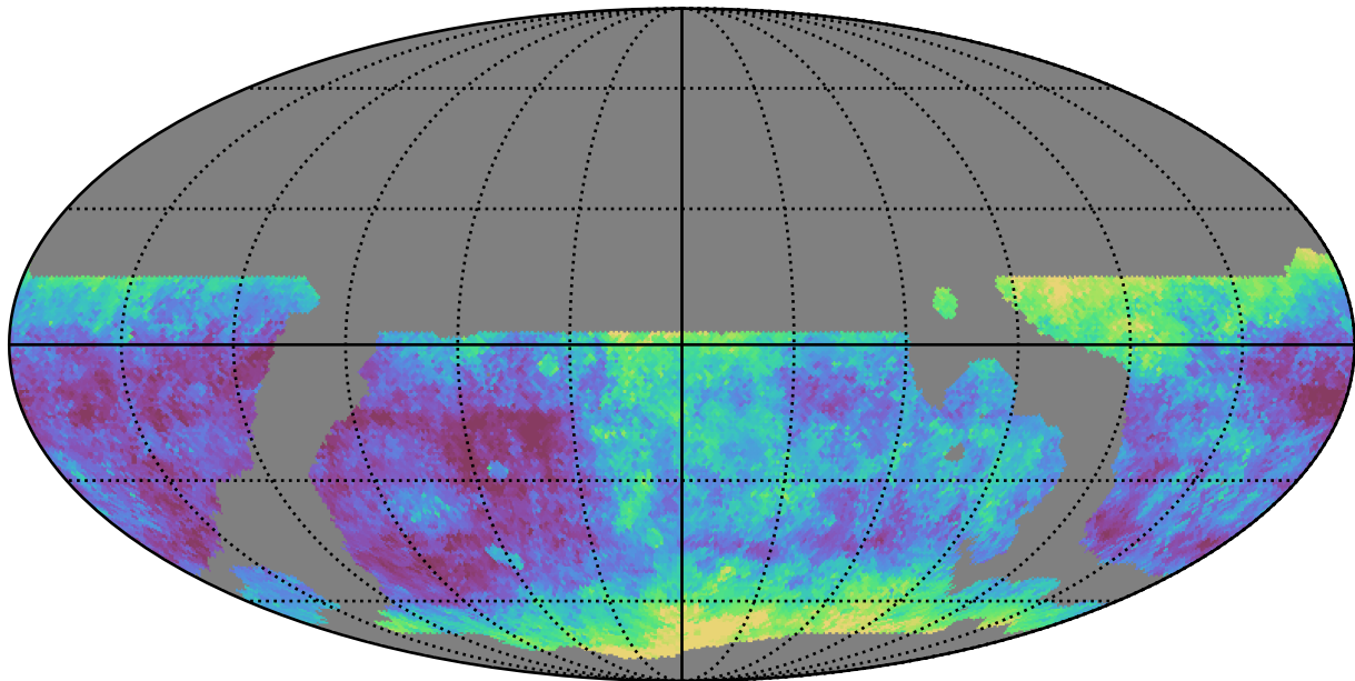
weather_cloudso4v3.4_10yrs WFD g band: Median seeingEff
