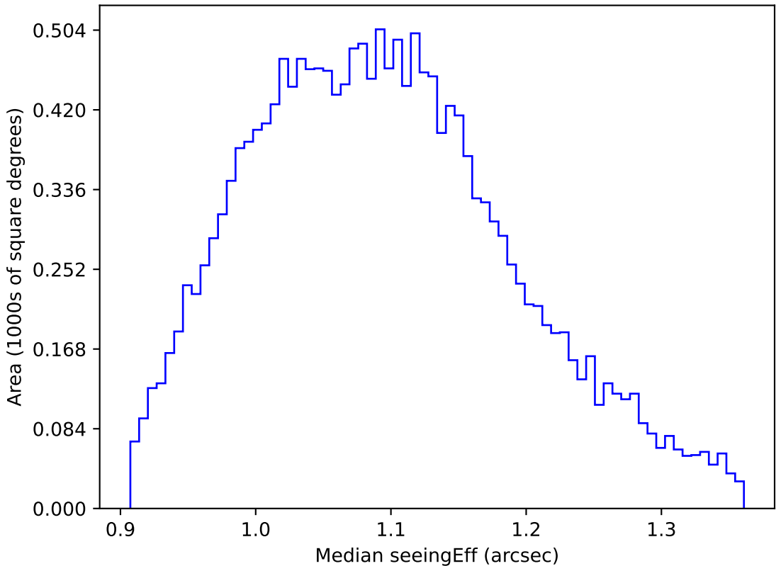
weather_cloudso4v3.4_10yrs WFD g band: Median seeingEff
